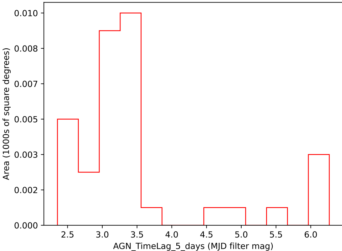
too_10_1v3.4_10yrs i band: AGN_TimeLag_5_days
