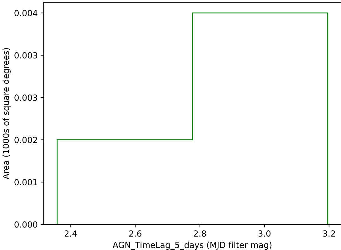
too_10_1v3.4_10yrs g band: AGN_TimeLag_5_days
