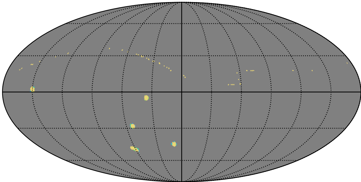
too_10_1v3.4_10yrs all bands: AGN_TimeLag_5_days
