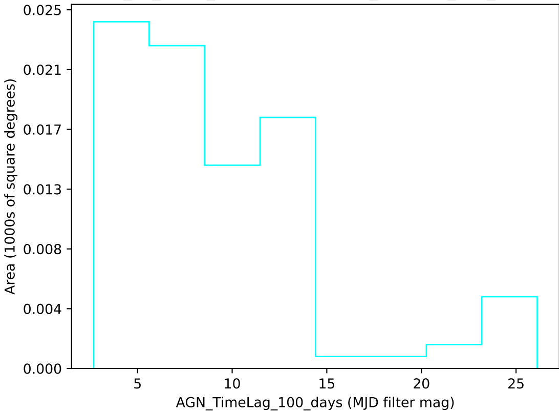
too_10_1v3.4_10yrs u band: AGN_TimeLag_100_days
