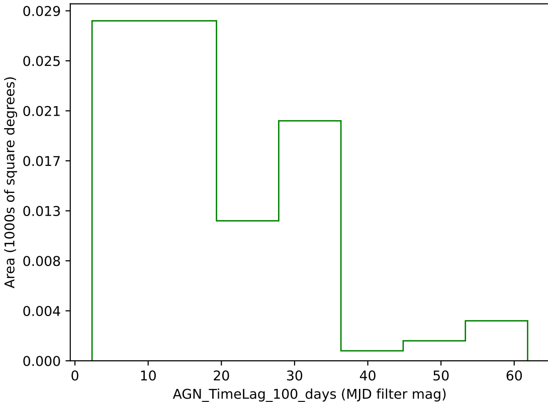
too_10_1v3.4_10yrs g band: AGN_TimeLag_100_days
