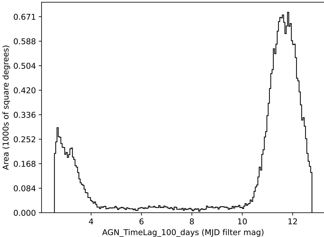
too_10_1v3.4_10yrs all bands: AGN_TimeLag_100_days
