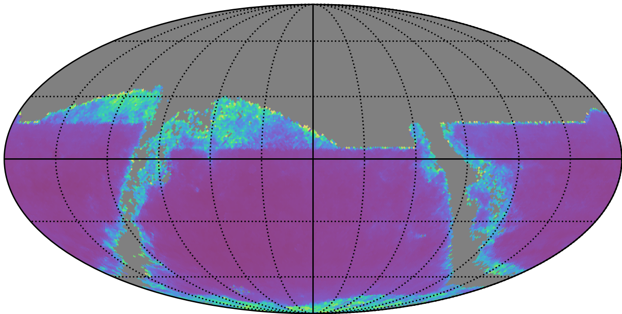
too_10_1v3.4_10yrs z band: AGN SF_uncert
