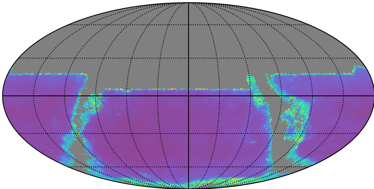
too_10_1v3.4_10yrs y band: AGN SF_uncert
