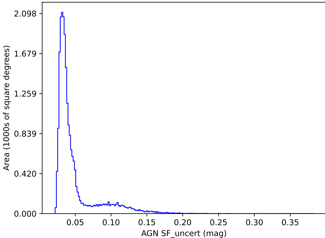
too_10_1v3.4_10yrs y band: AGN SF_uncert
