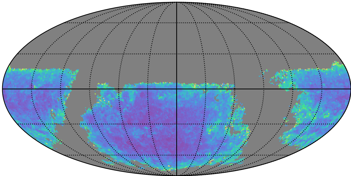
too_10_1v3.4_10yrs u band: AGN SF_uncert
