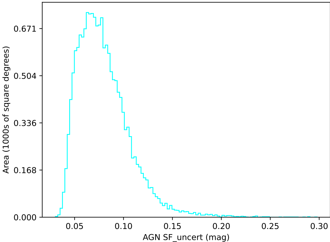
too_10_1v3.4_10yrs u band: AGN SF_uncert
