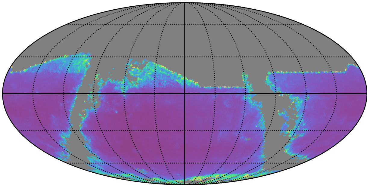
too_10_1v3.4_10yrs r band: AGN SF_uncert
