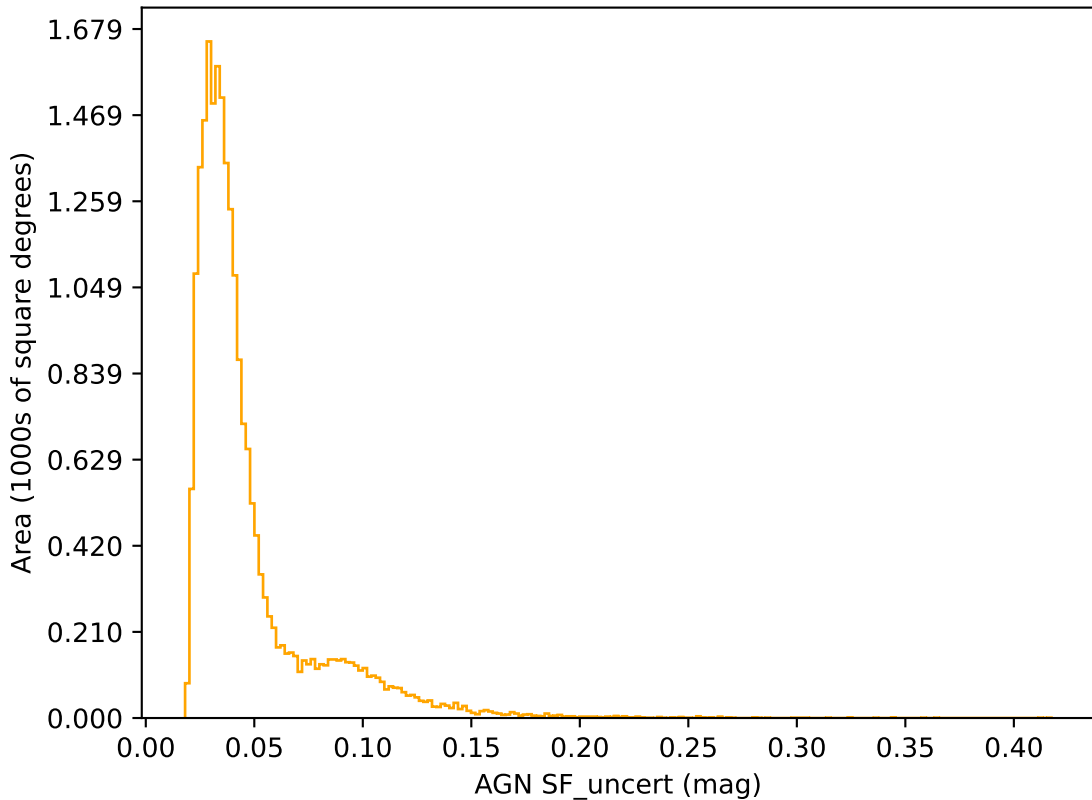
too_10_1v3.4_10yrs r band: AGN SF_uncert
