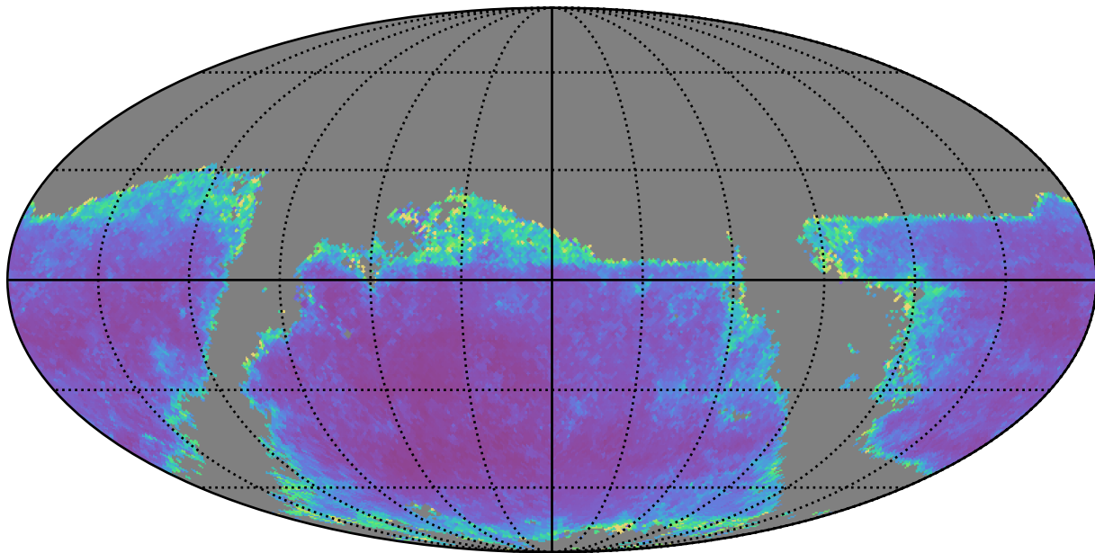
too_10_1v3.4_10yrs g band: AGN SF_uncert
