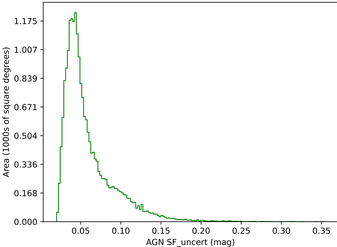
too_10_1v3.4_10yrs g band: AGN SF_uncert
