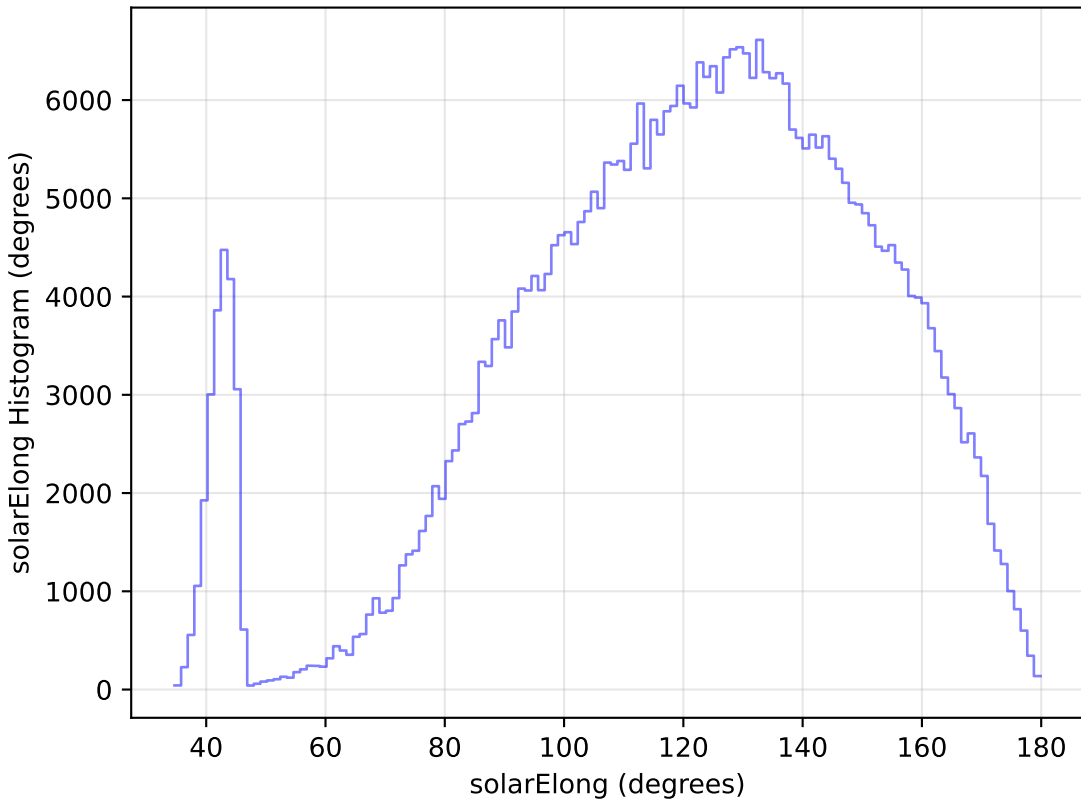
too_10_1v3.4_10yrs WFD z band: solarElong Histogram
