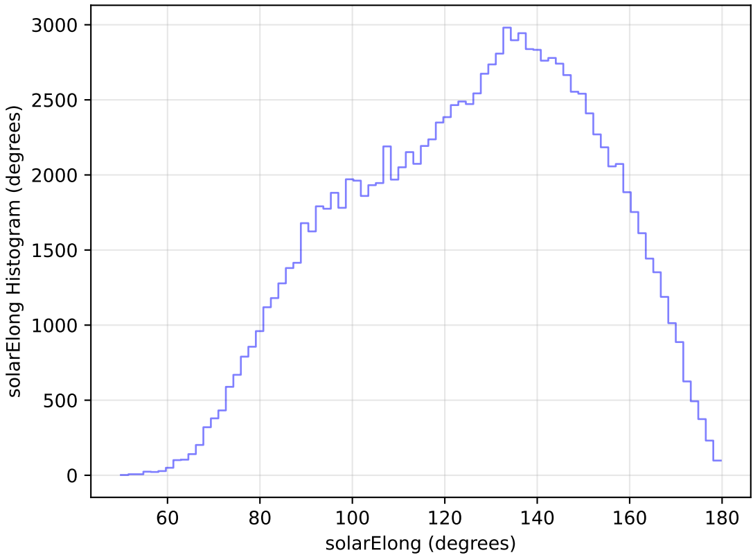
too_10_1v3.4_10yrs WFD u band: solarElong Histogram
