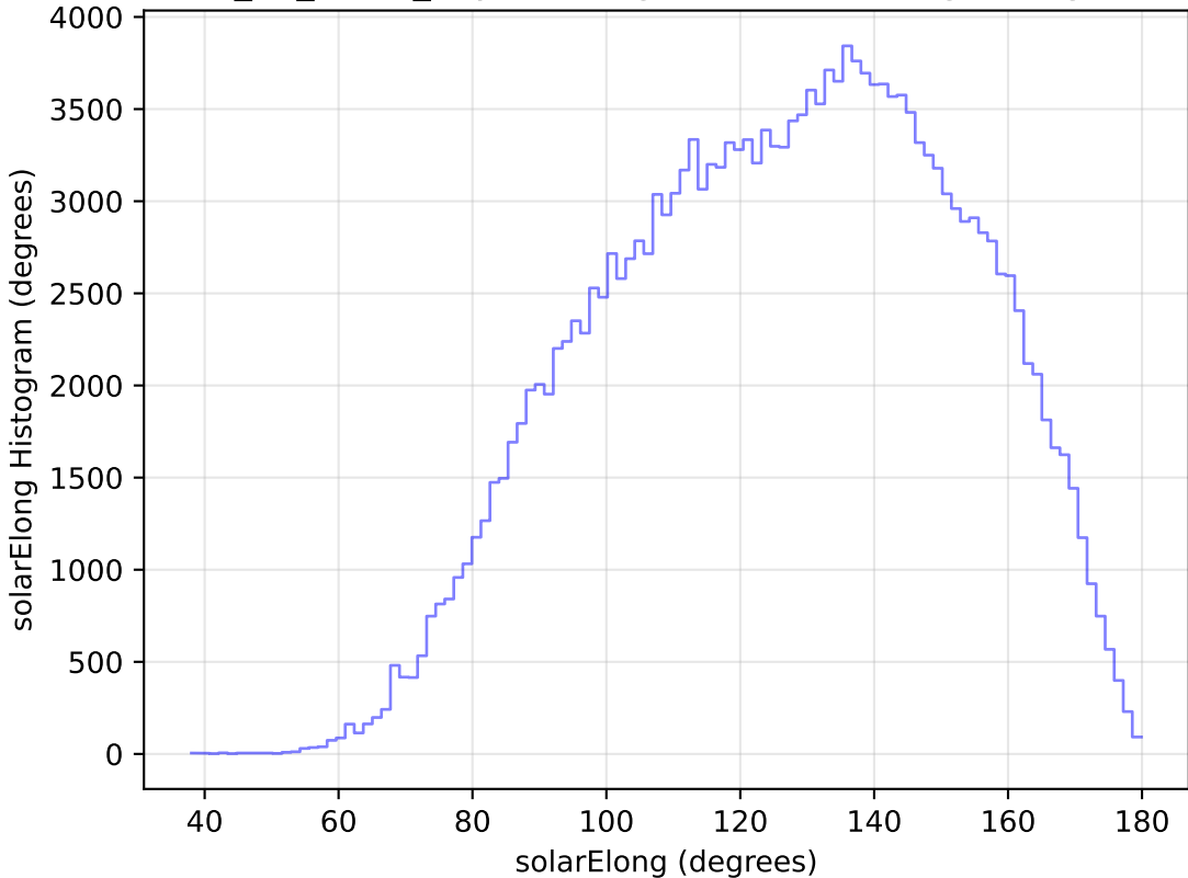
too_10_1v3.4_10yrs WFD g band: solarElong Histogram
