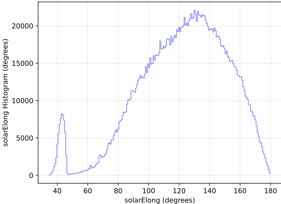
too_10_1v3.4_10yrs WFD all bands: solarElong Histogram
