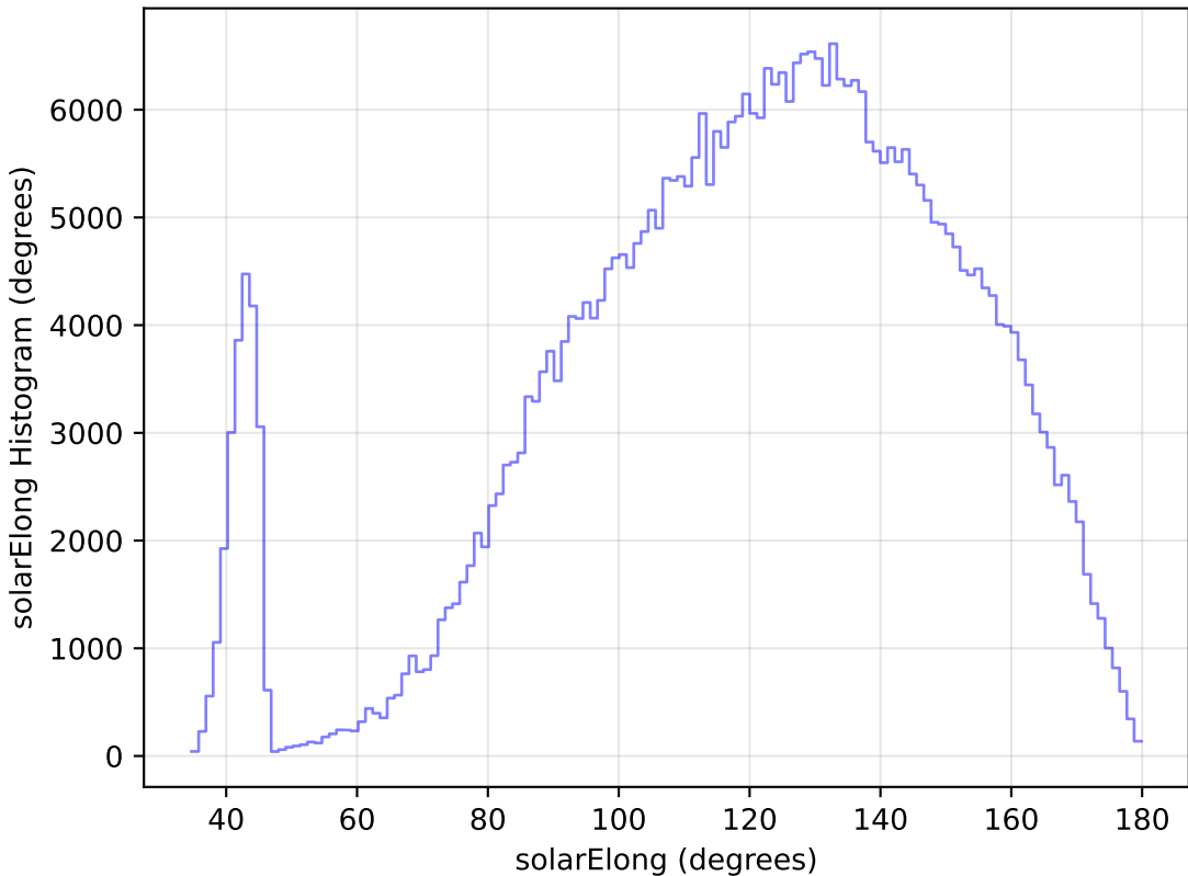
too_10_1v3.4_10yrs All sky z band: solarElong Histogram
