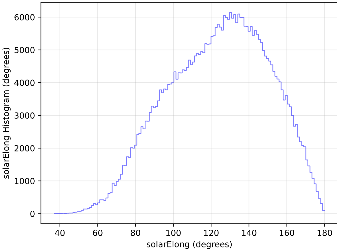
too_10_1v3.4_10yrs All sky y band: solarElong Histogram
