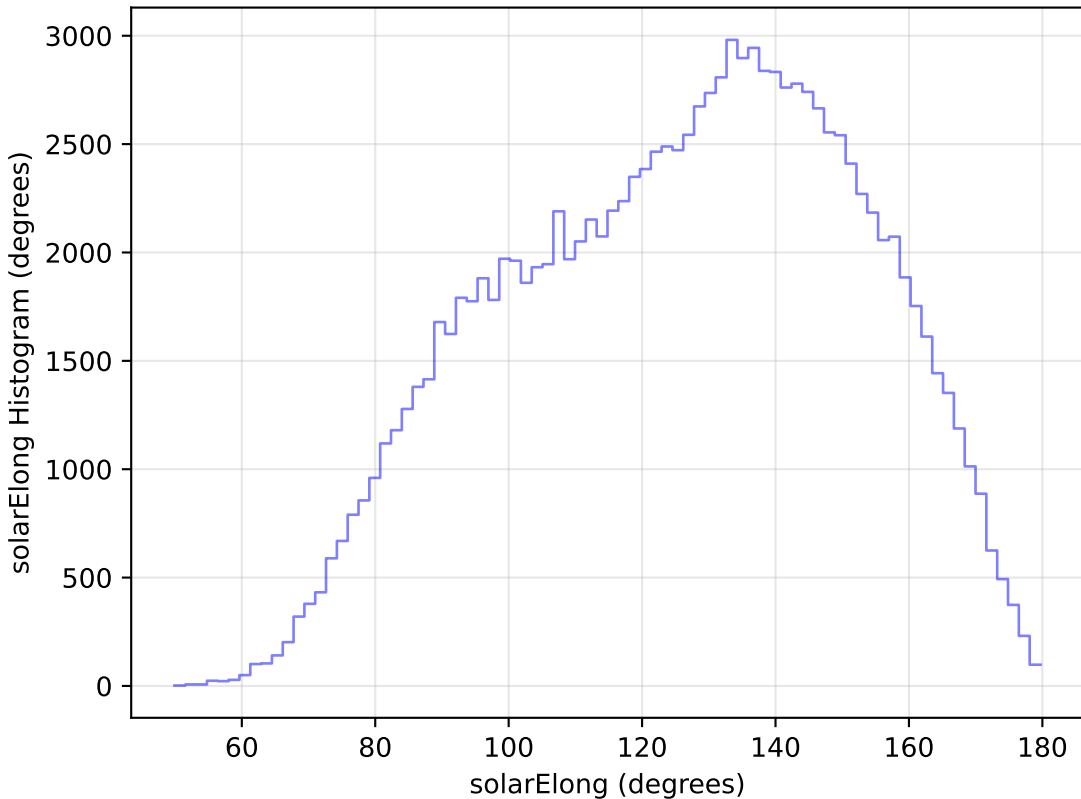
too_10_1v3.4_10yrs All sky u band: solarElong Histogram
