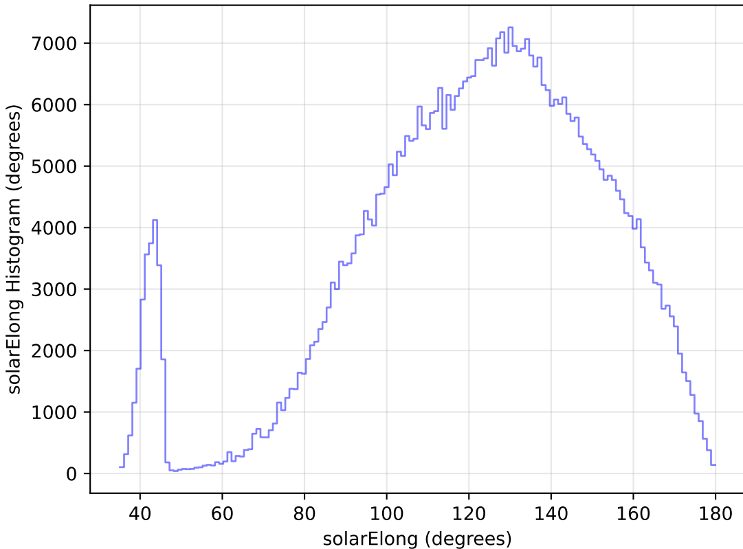
too_10_1v3.4_10yrs All sky i band: solarElong Histogram
