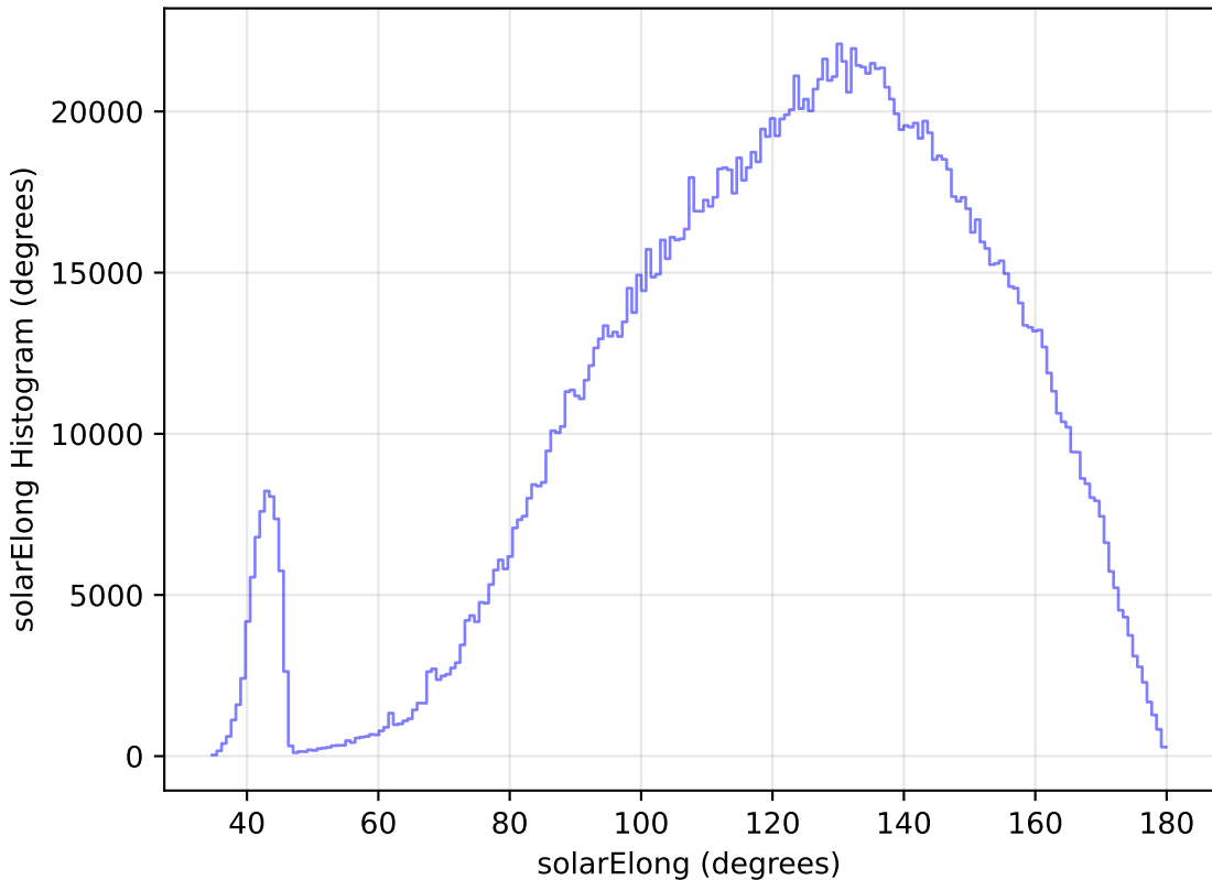
too_10_1v3.4_10yrs All sky all bands: solarElong Histogram
