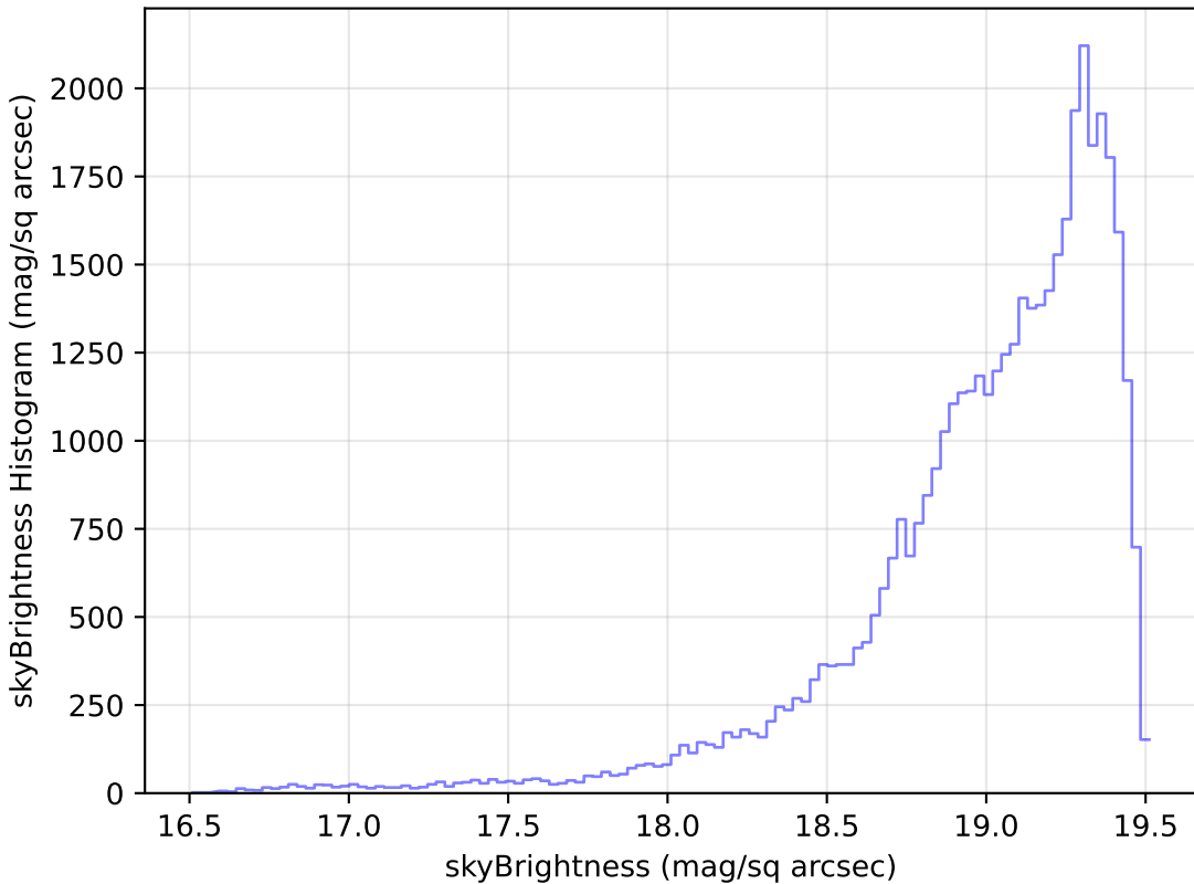
too_10_1v3.4_10yrs Yr 1 z band: skyBrightness Histogram
