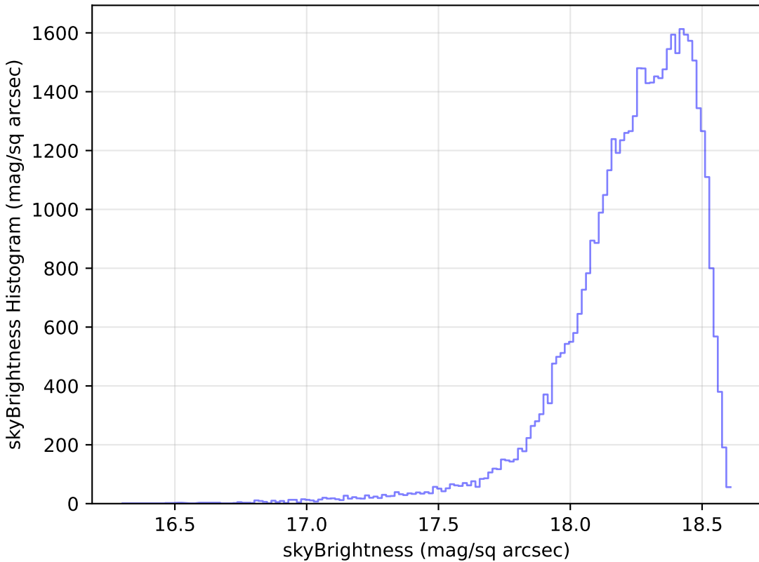
too_10_1v3.4_10yrs Yr 1 y band: skyBrightness Histogram
