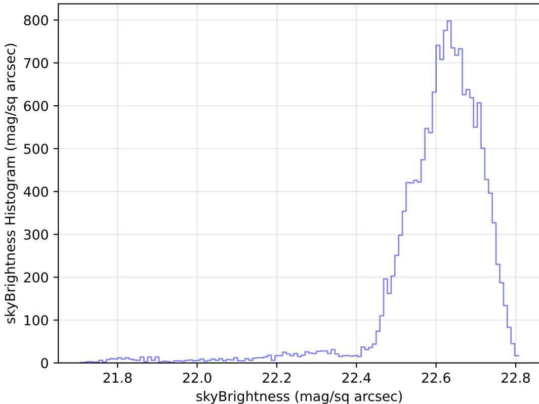
too_10_1v3.4_10yrs Yr 1 u band: skyBrightness Histogram
