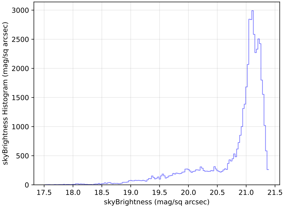
too_10_1v3.4_10yrs Yr 1 r band: skyBrightness Histogram
