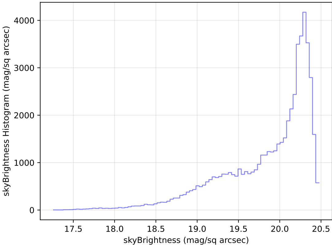
too_10_1v3.4_10yrs Yr 1 i band: skyBrightness Histogram
