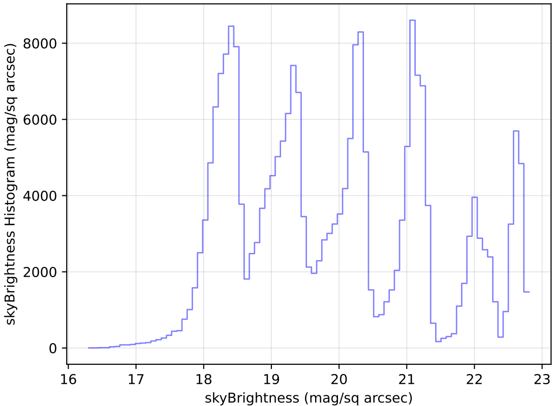
too_10_1v3.4_10yrs Yr 1 all bands: skyBrightness Histogram
