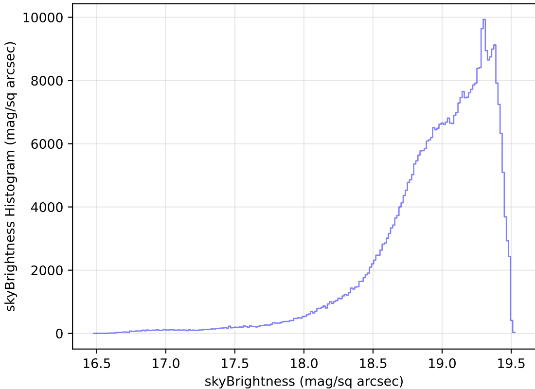
too_10_1v3.4_10yrs WFD z band: skyBrightness Histogram
