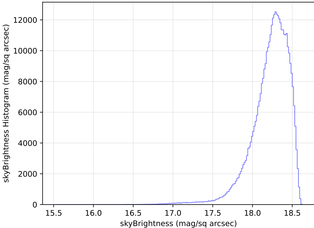
too_10_1v3.4_10yrs WFD y band: skyBrightness Histogram
