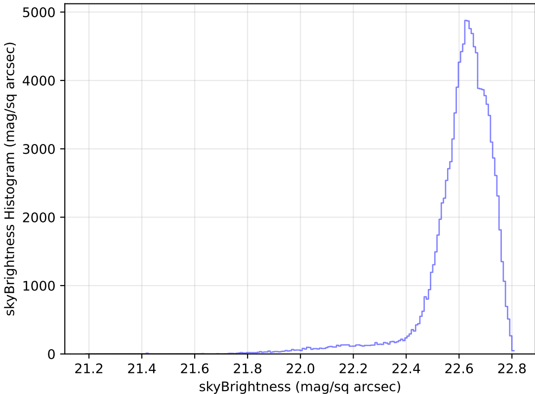
too_10_1v3.4_10yrs WFD u band: skyBrightness Histogram
