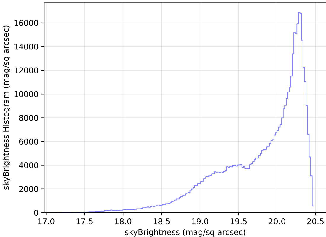
too_10_1v3.4_10yrs WFD i band: skyBrightness Histogram
