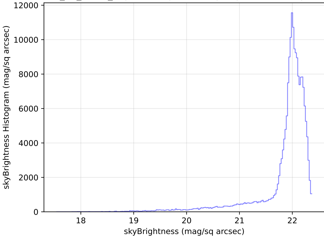
too_10_1v3.4_10yrs WFD g band: skyBrightness Histogram
