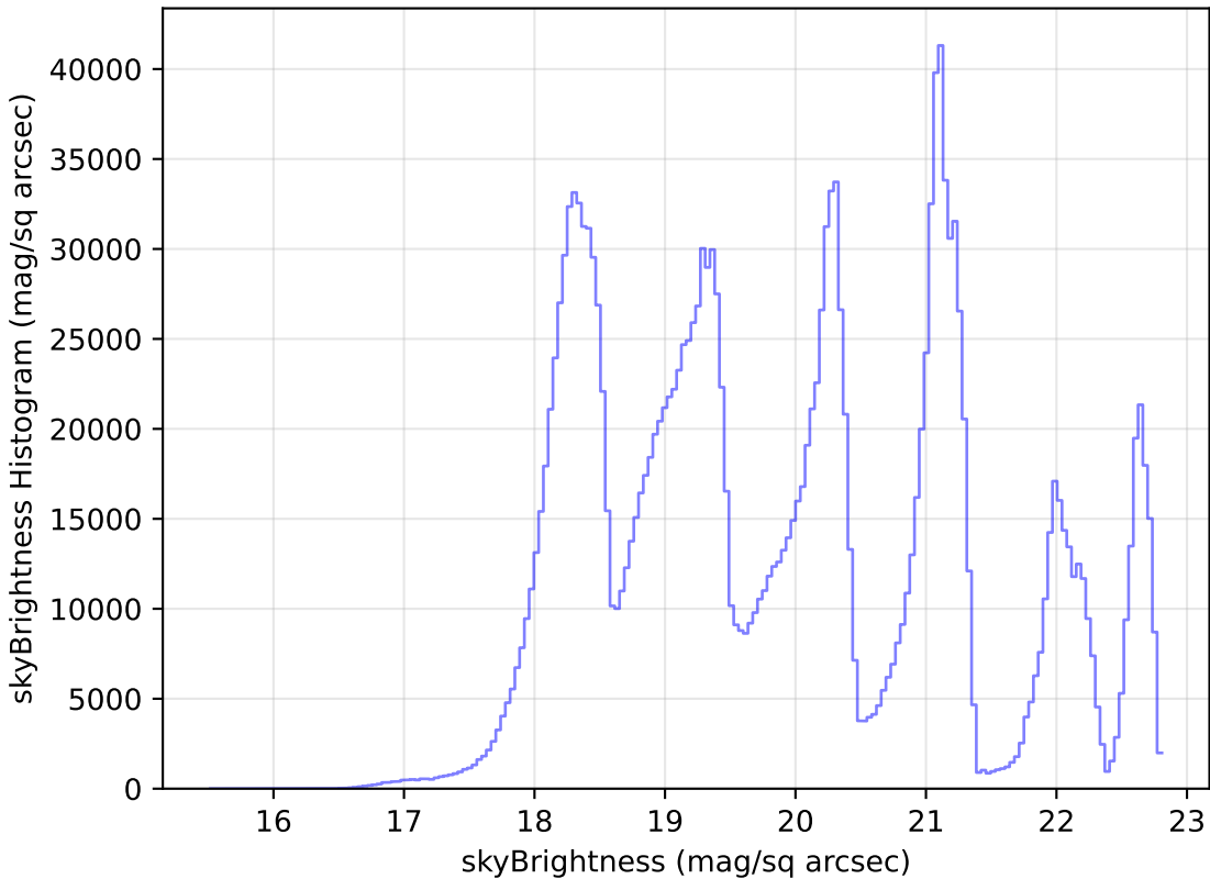
too_10_1v3.4_10yrs WFD all bands: skyBrightness Histogram
