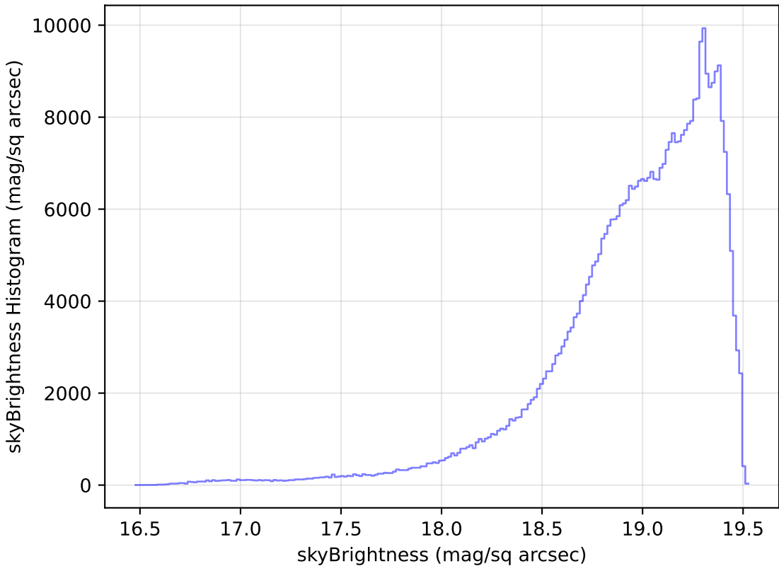
too_10_1v3.4_10yrs All sky z band: skyBrightness Histogram
