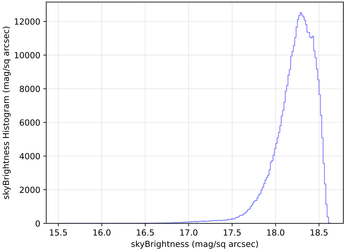
too_10_1v3.4_10yrs All sky y band: skyBrightness Histogram
