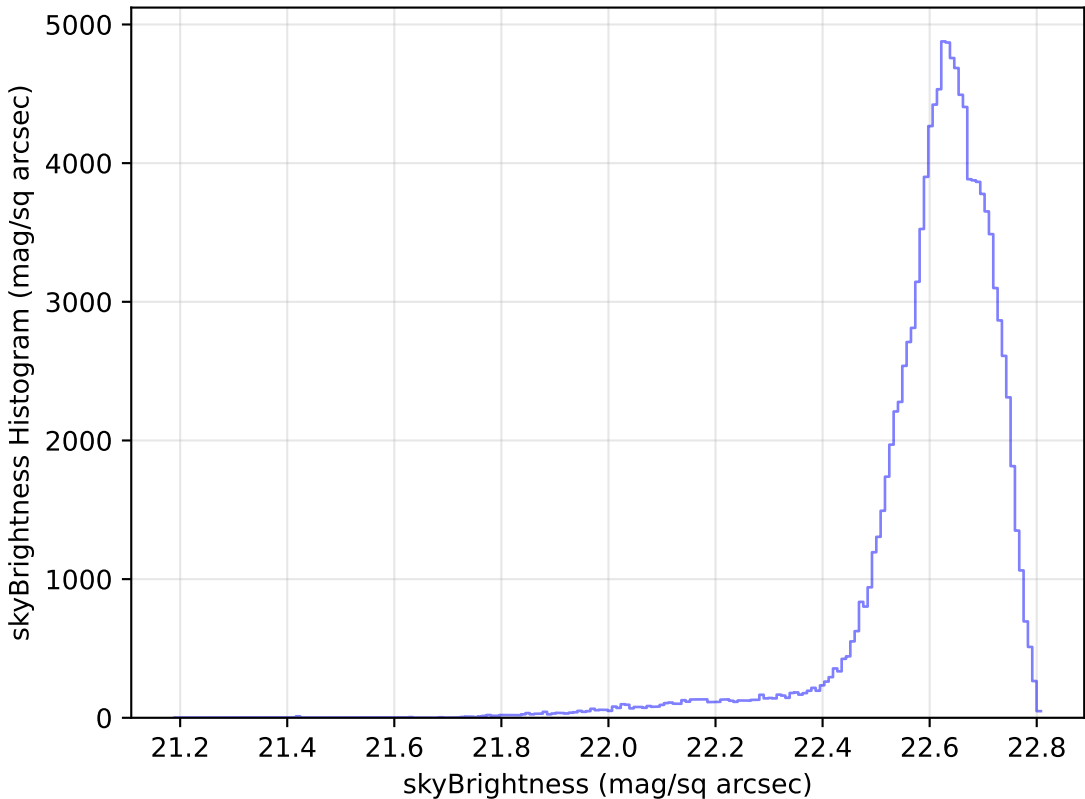
too_10_1v3.4_10yrs All sky u band: skyBrightness Histogram
