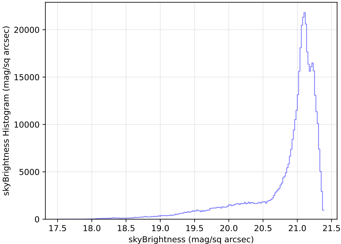
too_10_1v3.4_10yrs All sky r band: skyBrightness Histogram
