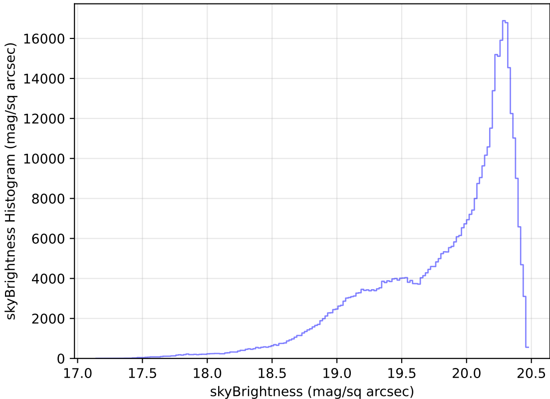
too_10_1v3.4_10yrs All sky i band: skyBrightness Histogram
