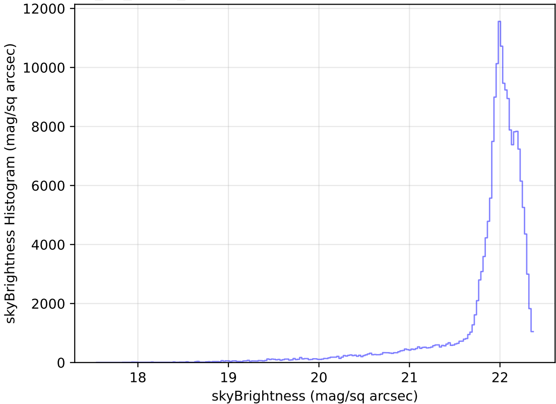
too_10_1v3.4_10yrs All sky g band: skyBrightness Histogram
