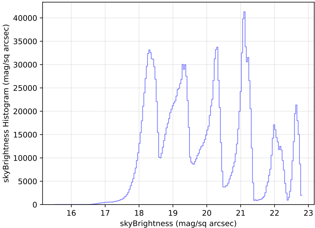
too_10_1v3.4_10yrs All sky all bands: skyBrightness Histogram
