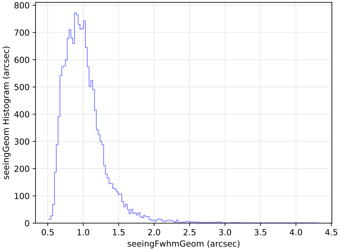
too_10_1v3.4_10yrs Yr 1 u band: seeingGeom Histogram
