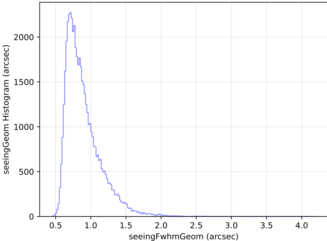
too_10_1v3.4_10yrs Yr 1 r band: seeingGeom Histogram
