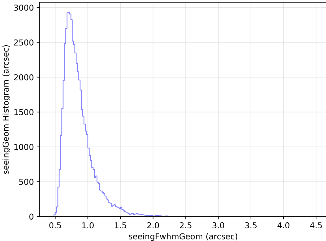
too_10_1v3.4_10yrs Yr 1 i band: seeingGeom Histogram
