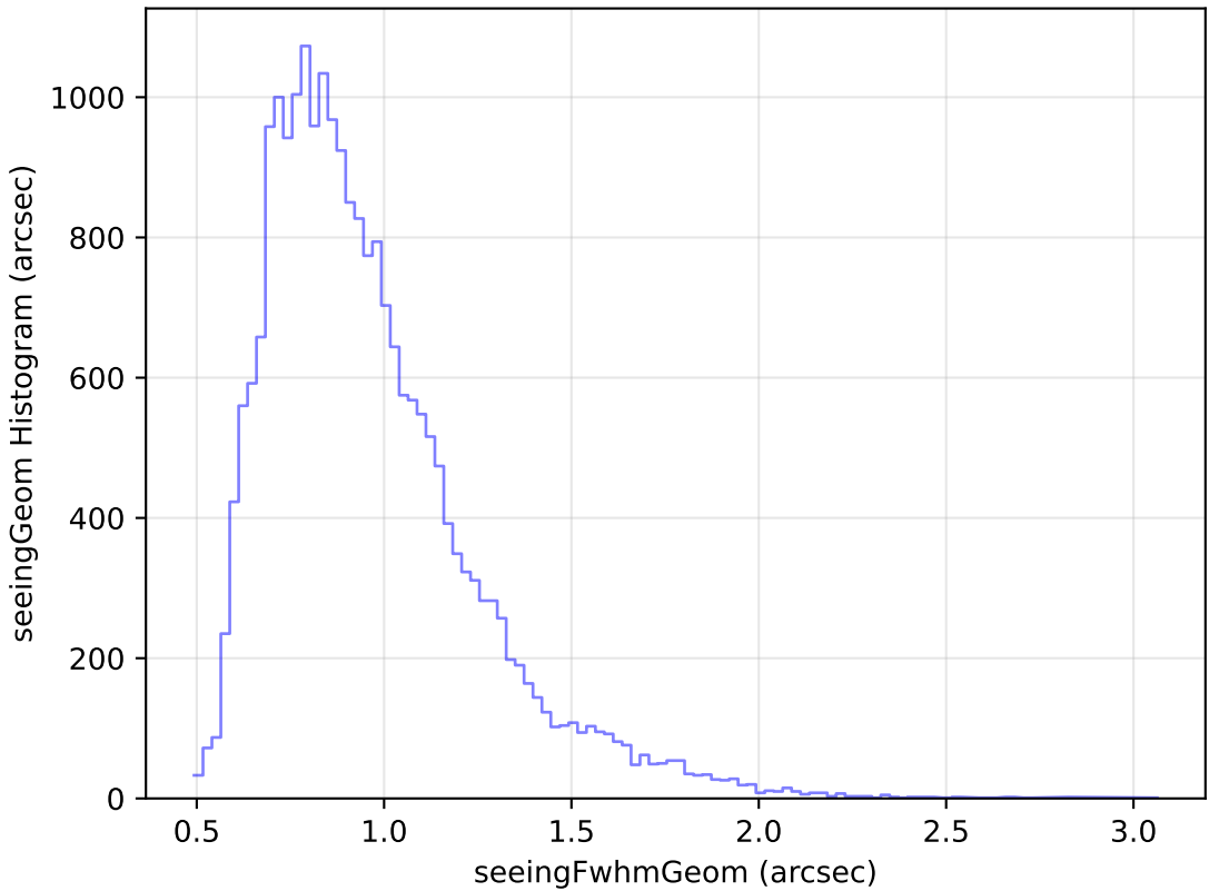
too_10_1v3.4_10yrs Yr 1 g band: seeingGeom Histogram
