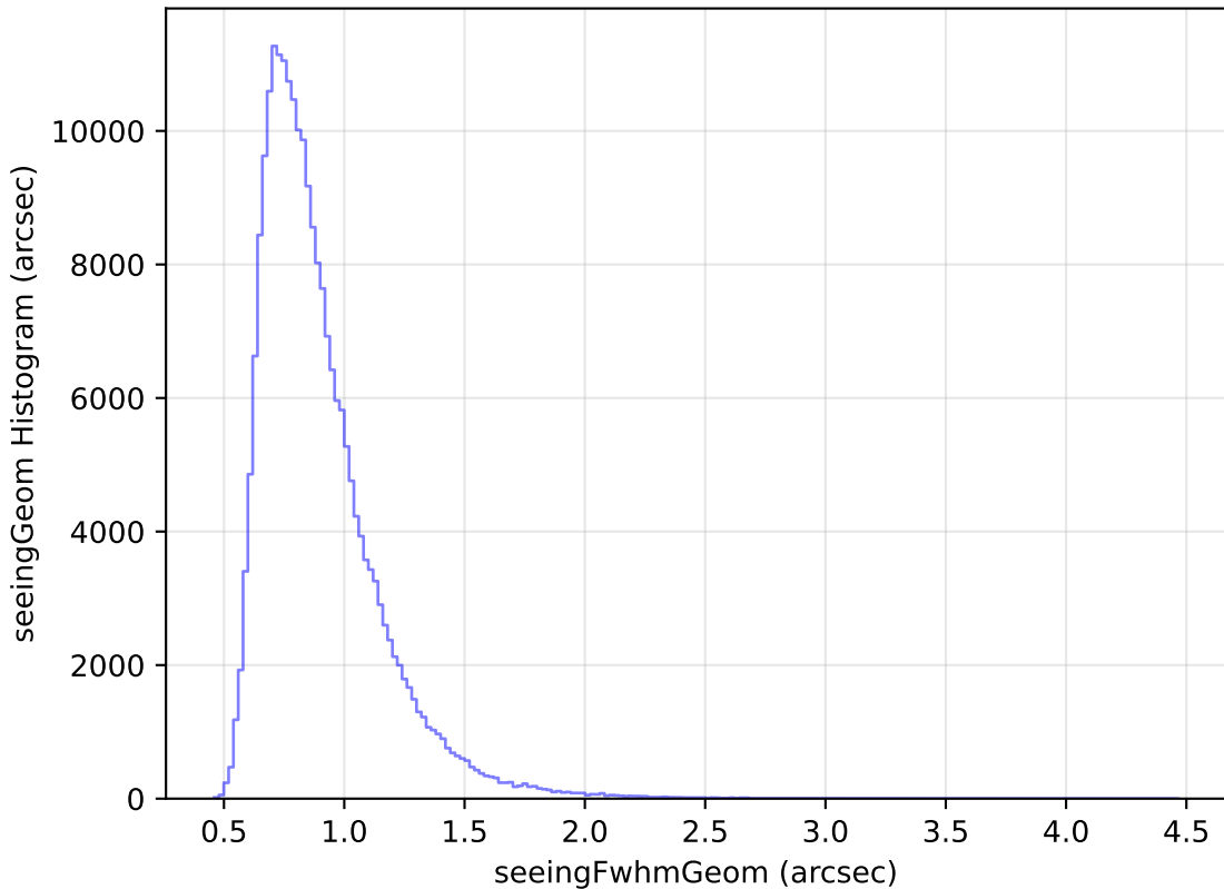
too_10_1v3.4_10yrs Yr 1 all bands: seeingGeom Histogram
