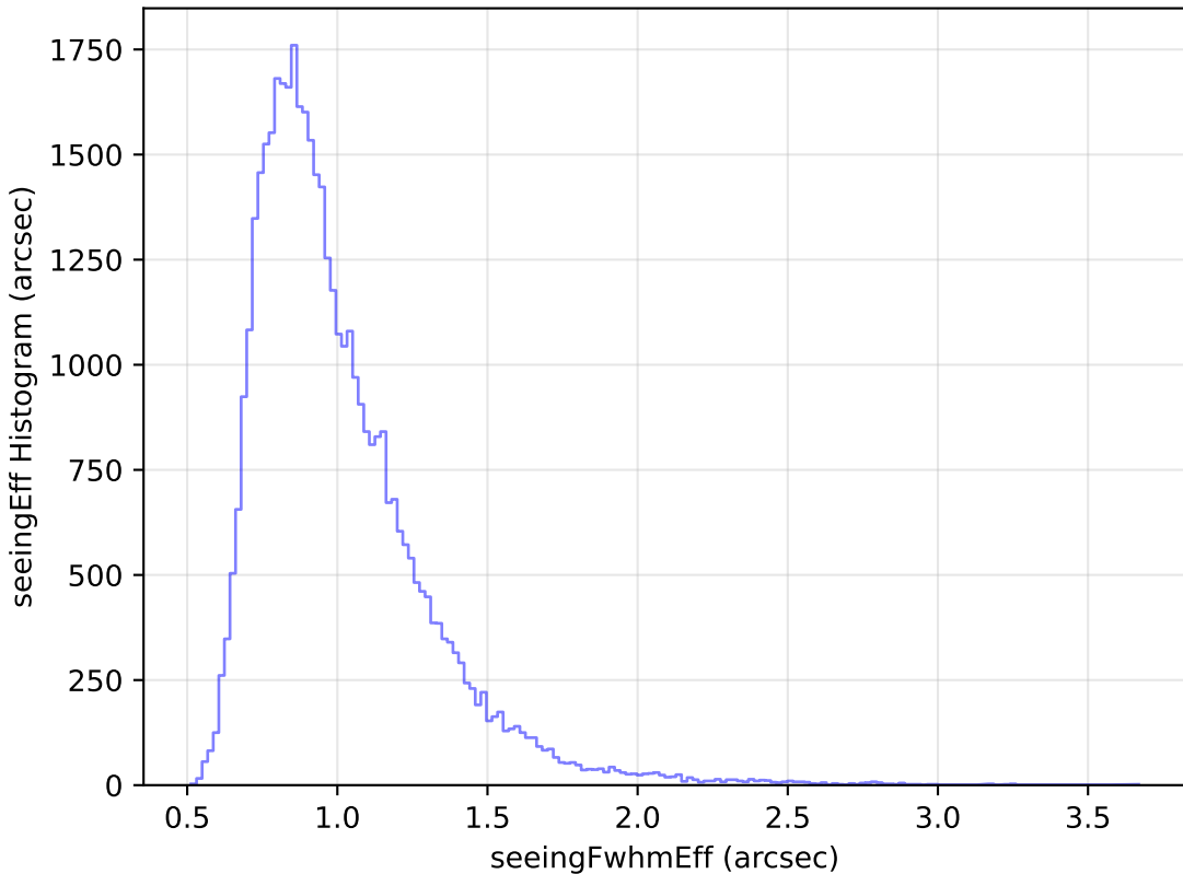
too_10_1v3.4_10yrs Yr 1 z band: seeingEff Histogram
