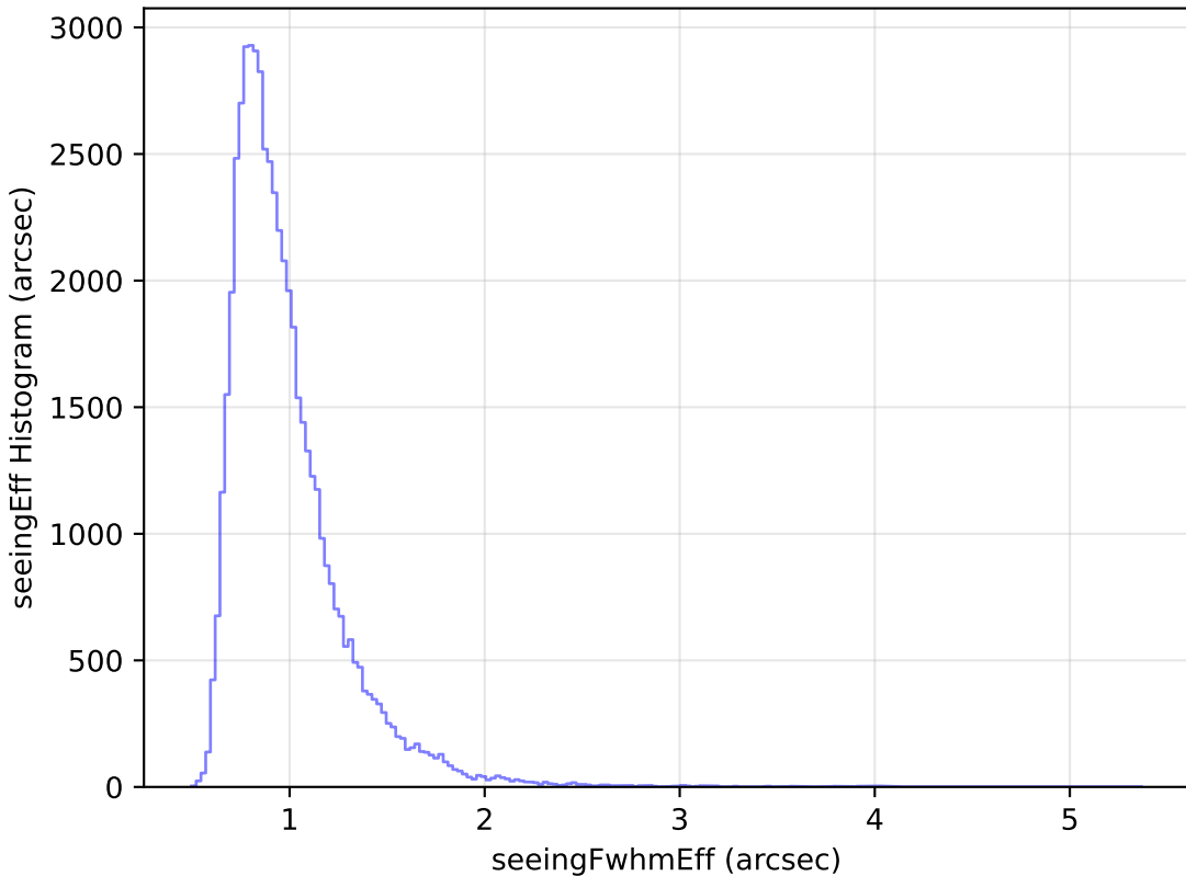
too_10_1v3.4_10yrs Yr 1 i band: seeingEff Histogram
